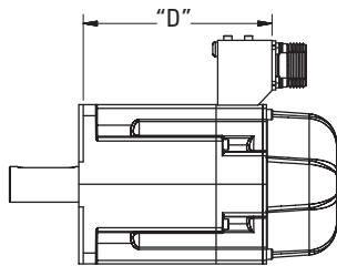
REAR CONNECTOR MOUNTING OPTION
